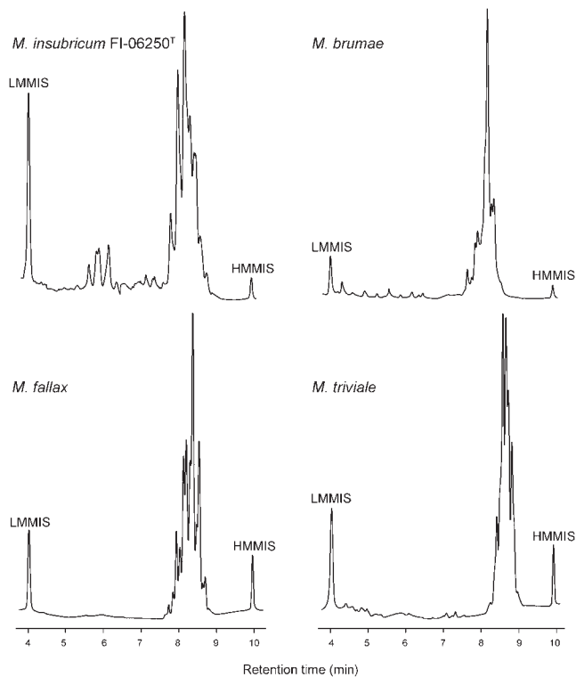
Fig. 1. HPLC patterns of mycolic acids of Mycobacterium insubricum sp. nov. FI-06250 T , M. brumae , M. fallax and M. triviale . LMMIS, Low-molecular-mass internal standard; HMMIS, high-molecular-mass internal standard. Patterns for reference species were taken from http://www.mycobactoscana.it .
