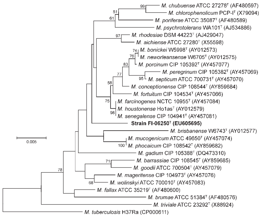
Fig. 3. Neighbour-joining phylogenetic tree based on 16S rRNA gene sequences. M. tuberculosis H37Ra was used as the outgroup. Bootstrap values \geq 50\% are reported at nodes. Bar, 0.5% sequence difference.
